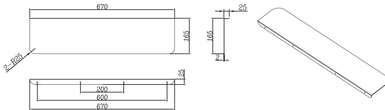
Metal Shelf Detail
